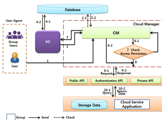
Fig. 2. Authentication Process
